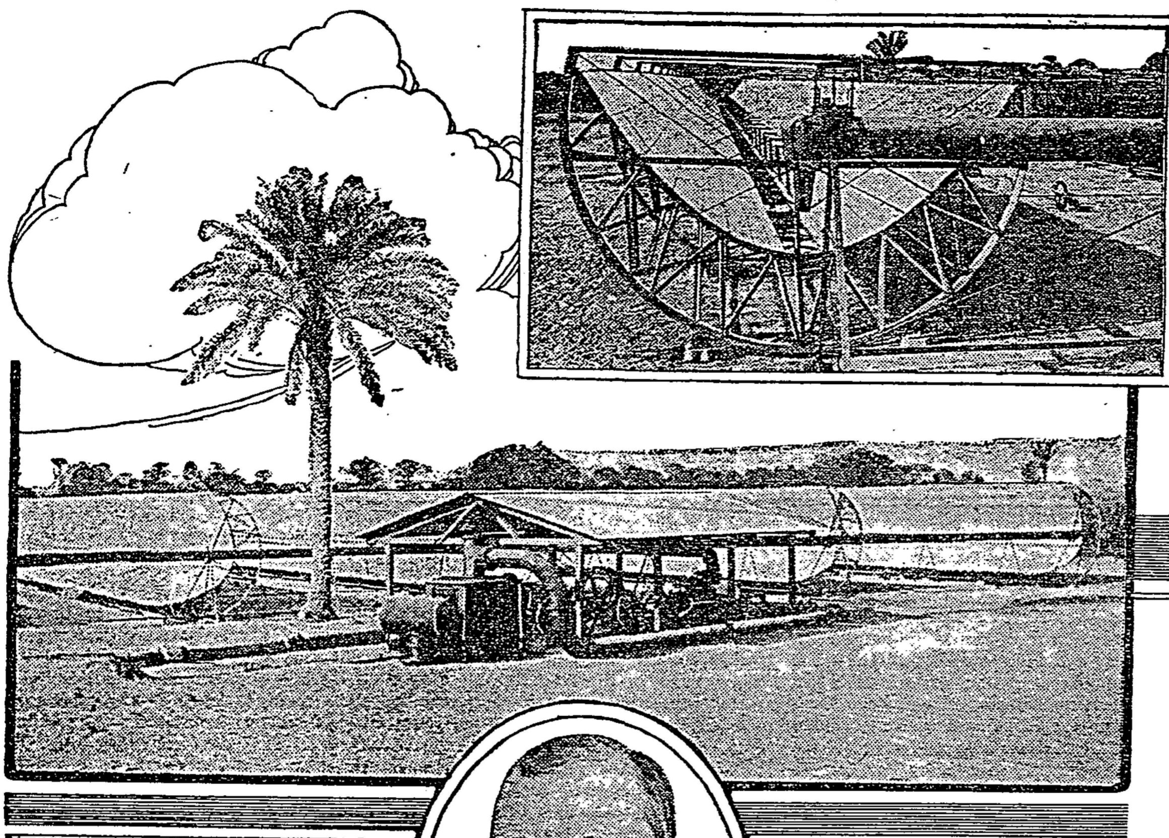
(Top Insert) End View of one of the five heat absorbers
